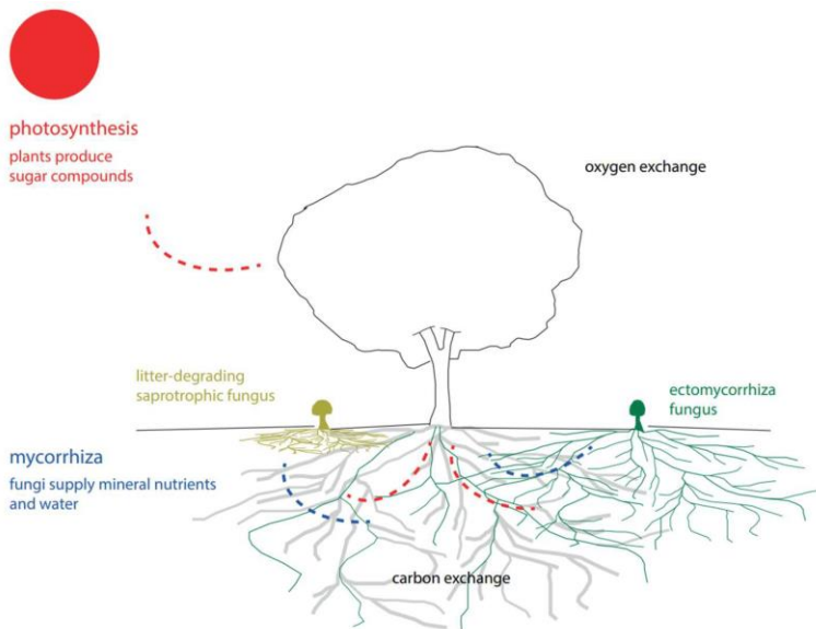
Figure 4: Schematic representation of mycorrhiza: Mutualistic association between tree roots and fungal mycelium [10].
