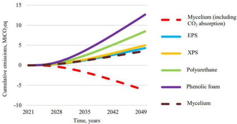
Figure 6: Accumulated GHG emissions throughout insulation material manufacturing [80].
