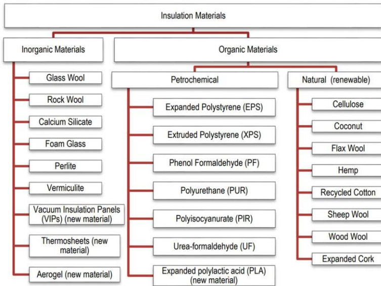
Figure 5: Classification of building insulation materials [40].
