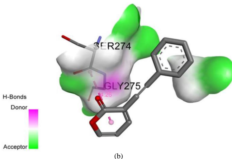
Figure 9: Molecular docking of SPD. (a) Binding pose of SPD molecular structure on DENV-2 E protein (PDB entry: 4u2c). Arrow indicates the molecular structure of SPD. Domain III is marked red. (b) Interaction of SPD with the amino acid residues of DENV-2 E protein as shown by docking. SPD binds at domain III of E protein which ranges from amino acid residues 274 to 275, by forming a hydrogen bond with the amino acid residues of the E protein.
