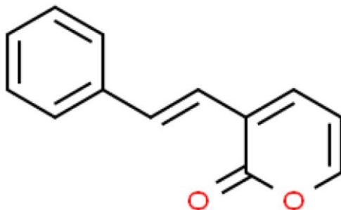
Figure 1: Basic structure of styrylpyrone.
