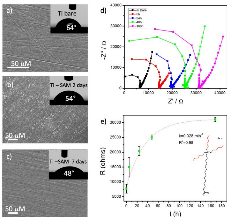
Figure 2: a-c) SEM micrographs of titanium bare surface, Ti-SAM of 3 after 2 days and after 7 days, respectively. Inset: contact angle images. d) Nyquist plots for Ti-SAM of 3 using agarose gel 1% as solid electrolyte. The frequency range was 0.1 Hz to 100 MHz, frequency increases from right to left, excitation signal of 25 mV peak amplitude was applied at OCP vs. Platinum wires as reference and counter electrode. e) Resistance (Ohms) vs time (hours) adsorption isotherm fit for the set of data.
