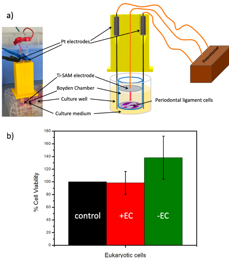
Figure 5: a) 3D imprinted device for the realization of the tests on eukaryotic cells. The Ti-SAM electrode is in contact with cells in the Boyden chamber, while the two Pt electrodes pass through the holes in culture well. b) % Cell viability of eukaryotic cells with and without electrochemical activation of 3-modified titanium surfaces.
