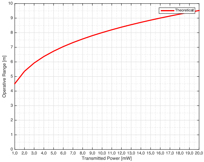
Figure 7: Assessment of the operative range vs. transmitted power in controlled environment.
