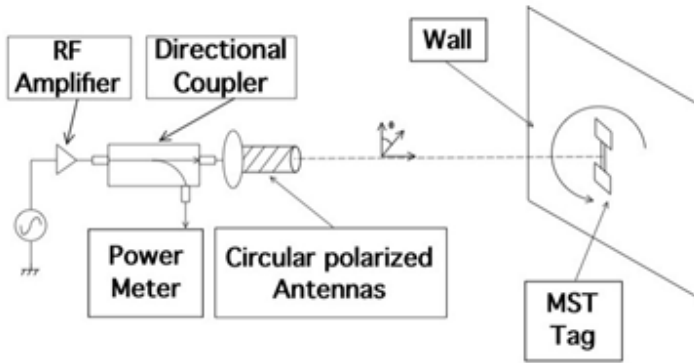
Figure 8: Assessment of the tag received signal vs. tag orientation. Experimental set-up.
