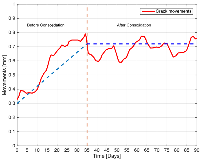
Figure 16: Crack movements vs. time. The tag placed on position B in the north side of the building, before and after the consolidation.
