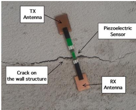
Figure 11: Photo of the crack and the tag placed on position A West side of the building. Photo of the considered experimental scenario, a 110 years old building under renovation.
