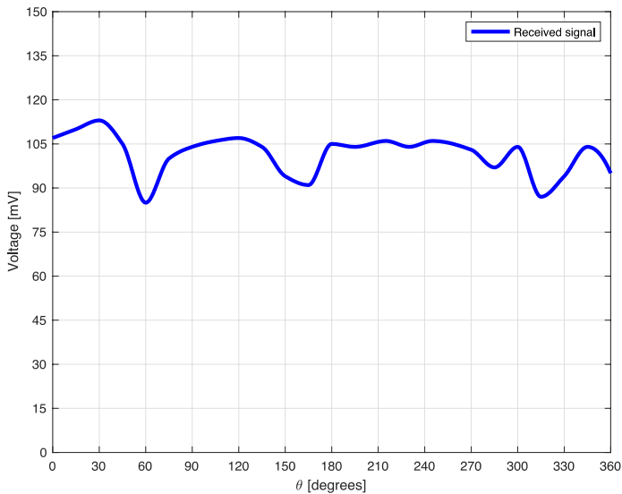
Figure 9: Assessment of the tag received signal vs. tag orientation. Measured signal vs tag orientation.
