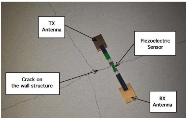
Figure 12: Photo of the crack and the tag placed on position B North side of the building.
