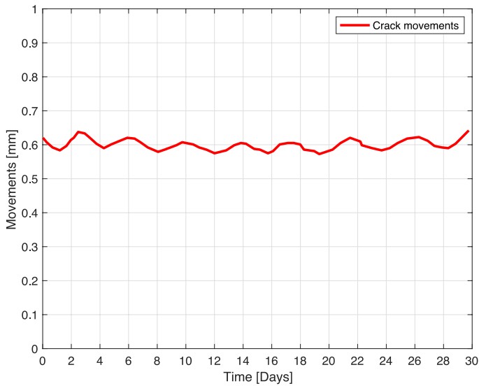
Figure 17: Crack movements vs. time. The tag placed on position C in the north side of the building, showing a safe situation.
