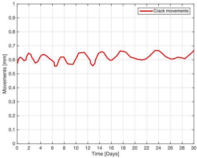
Figure 13: Crack movements vs. time. The tag placed in position A in the west side of the building.
