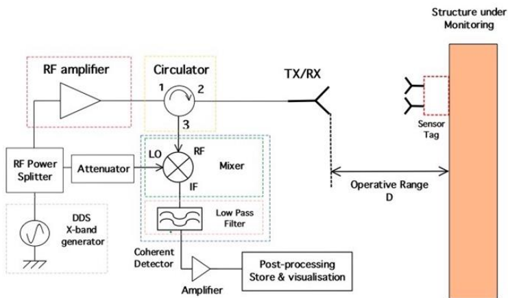
Figure 3: Reader Schema.
