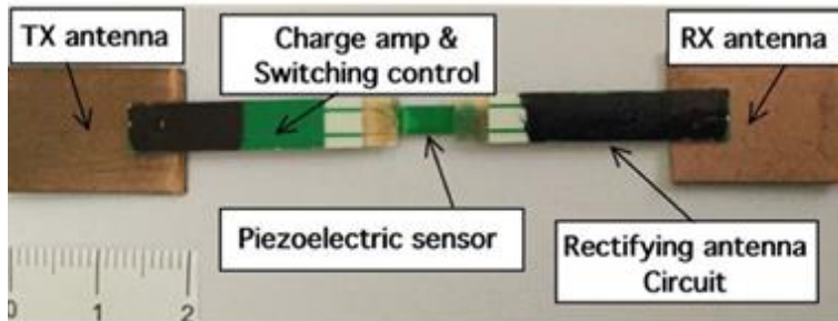
Figure 5: Tag photo.
