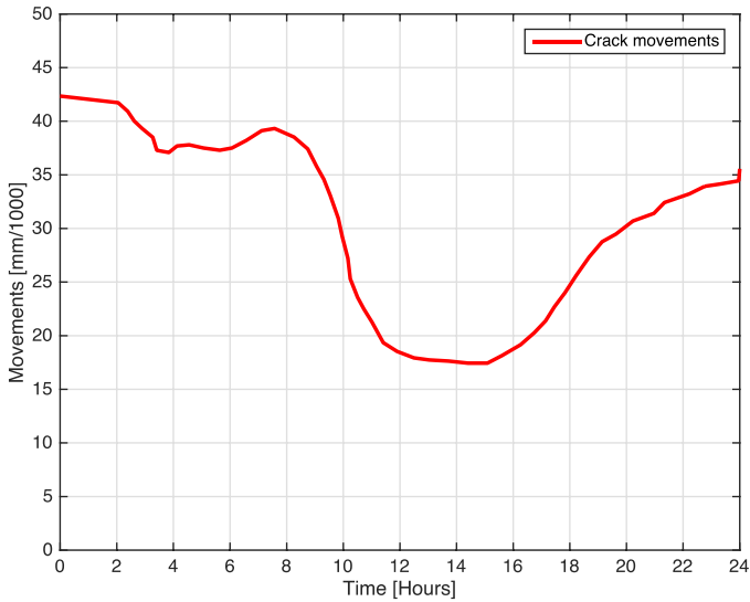
Figure 14: Crack movements vs. time. One day measurement showing the small movement due to temperature changes. Tag placed in position A.
