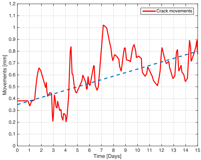
Figure 15: Crack movements vs. time. The tag placed on position B in the north side of the building, showing a dangerous situation with possible collapse.
