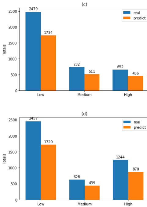
Figure 4: Real vs. predicted values with RF classifier for each dataset, using labels ‘low’, ‘medium’, and ‘high’ for the dependent variables. The figure shows the total values of the real versus the classified values: part a) with dataset A1; part b) with dataset A2; part c) with dataset B1; and part d) with dataset B2.
