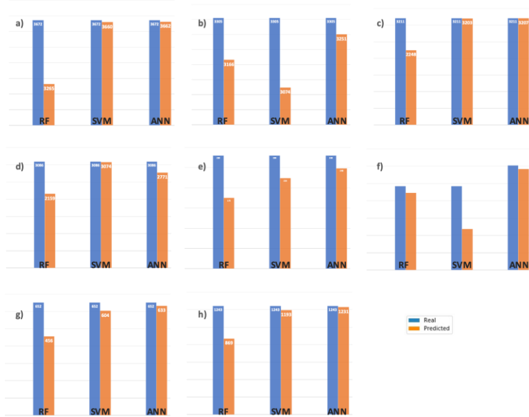
Figure 6: Comparison of real vs predicted values for each dataset, considering the labels ‘low’ and ‘high’ for each dataset and each of the algorithms used (RF, SVM and ANN). Data distribution: a) ‘low’ with dataset A1, b) ‘low’ with dataset A2, c) ‘low’ with dataset B1, d) ‘low’ with dataset B2, e) ‘high’ with dataset A1, f) ‘high’ with dataset A2, g) ‘high’ with dataset B1, and h) ‘high’ with dataset B2.
