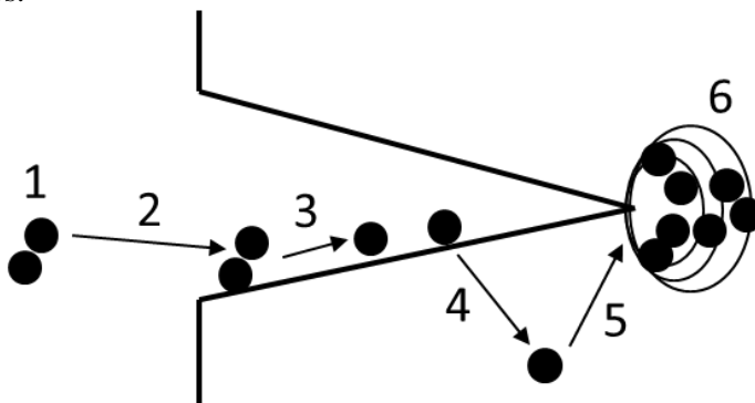
Figure 6: Rate-limiting steps for the transport of hydrogen to the fracture propagation zone, adapted from [59]. Here, 1 = transport of hydrogen to the crack tip; 2 = physical adsorption; 3 = dissociative chemical adsorption; 4 = hydrogen absorption; 5 = transport of hydrogen to regions of tensile stress; and 6 = hydrogen material interactions.
